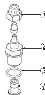
INJECTION 59837-I
