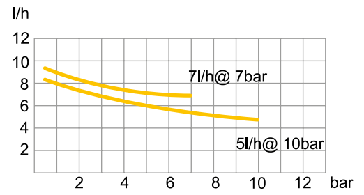
Models with automatic purge
